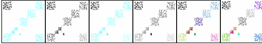
Fig. 3. Sequence of clusters generated by the ANN. Total number of points 774. Each colour represents a different cluster that was found.
