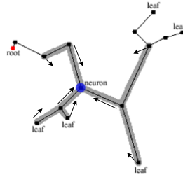
Fig. 2. Subtree for neuron falling within 2 links
