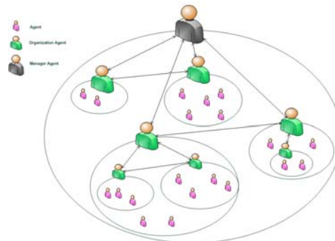
Figure 3. OrganizationManager and OrganizationAgents !
