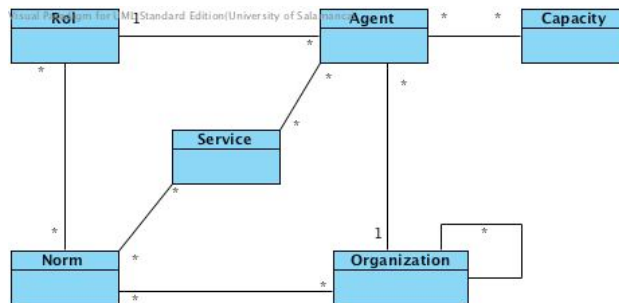
Figure 1. Principal classes of the system
