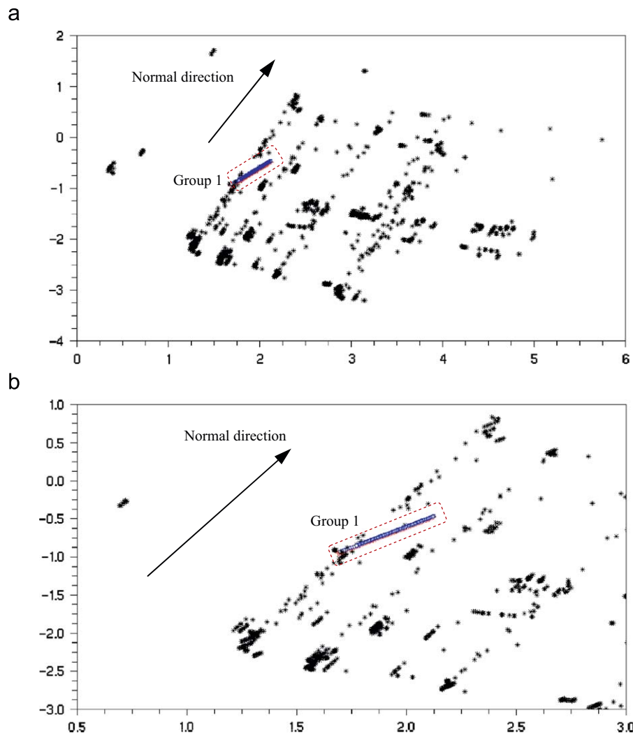
Fig. 5. CMLHL projections on the dataset involving on-line traffic analysis. (a) Projection of the first two components of the whole dataset by CMLHL and (b) zoomed portsweep attack (from Fig. 5a).
