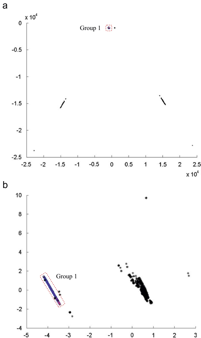
Fig. 6. Comparative projections of PCA and LDA on the dataset involving on-line traffic analysis. (a) PCA projection (through the two first principal components) and (b) LDA projection.
