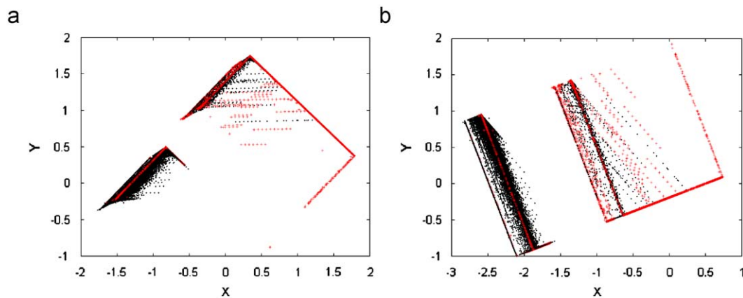
Fig. 9. Comparative projections on the dataset involving off-line traffic analysis. (a) PCA projection of the off-line analysis dataset and (b) LDA projection of the off-line analysis dataset.
