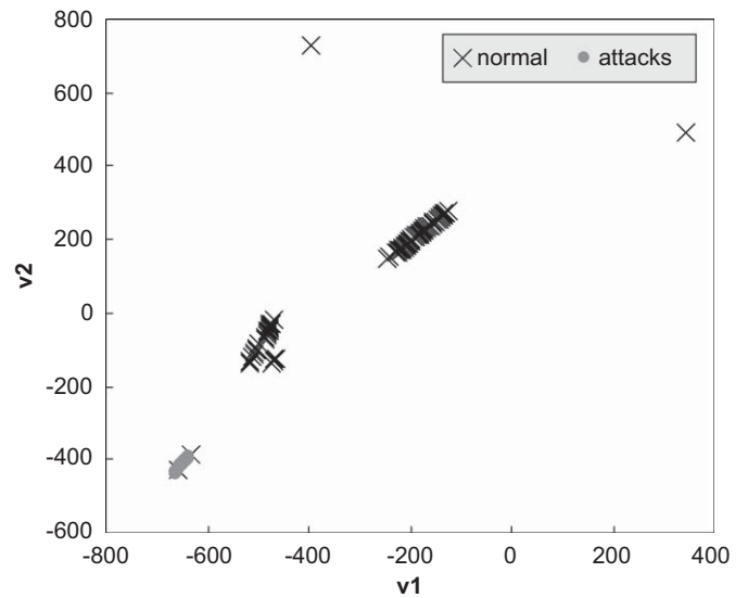
Fig. 7. AABP projection on the dataset involving on-line traffic analysis.
