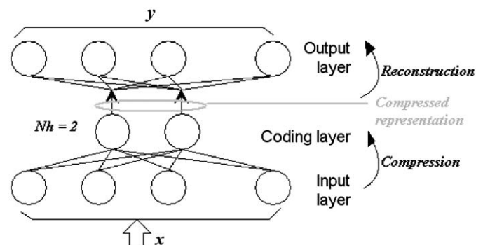
Fig. 1. A three-layer AABP network supports a lossy compression of input data.
