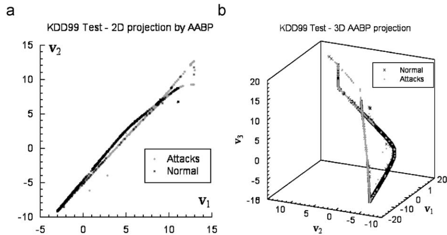
Fig. 8. AABP projections on the dataset involving off-line traffic analysis. (a) Two-dimensional projection and (b) three-dimensional projection.
