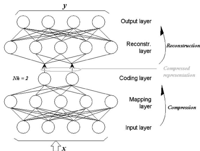
Fig. 2. A non-linear auto-associative back-propagation network includes five layers to reduce data dimensionality.
